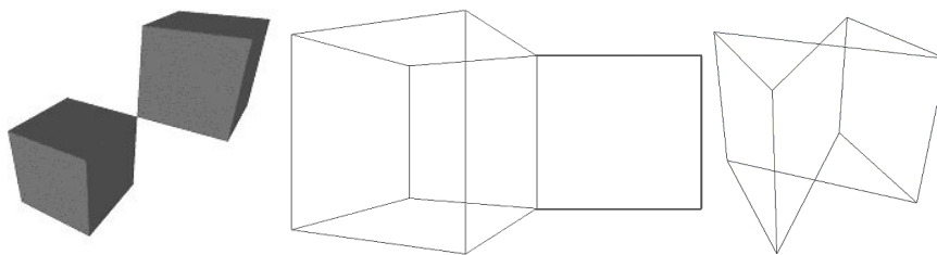
Fig. 5 Invalid objects with a non-2-manifold vertex (left, should be modelled as two objects), dangling face (centre) and intersecting faces (right).
