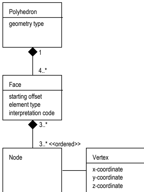
Fig. 4 UML diagram describing the storage of the polyhedron primitive and example.
