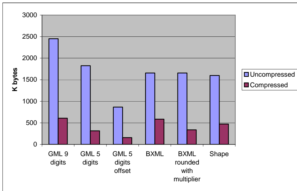
Figure 6: Compression of GML and variants (see Table 1 )
